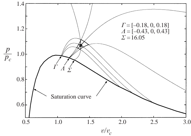
FIGURE 14. The region of \Gamma , A and \Sigma for a van der Waals gas with R/c_v = 0.02 where the composite solution is valid.
