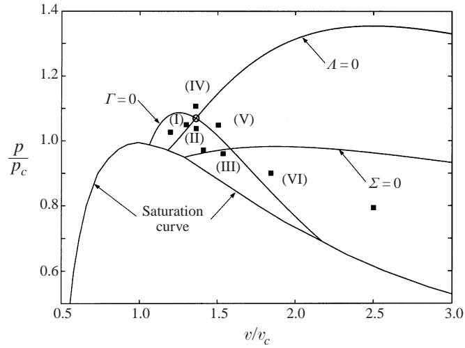
FIGURE 10. The map of \Gamma , \Lambda and \Sigma for a van der Waals gas with R/c_v = 0.02 .
